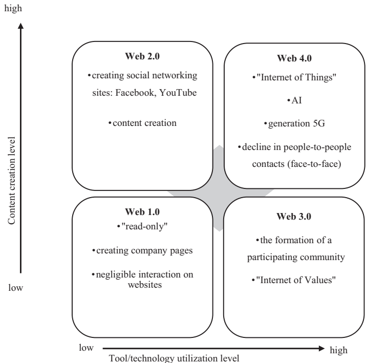
Figure 2. Internet evolution
